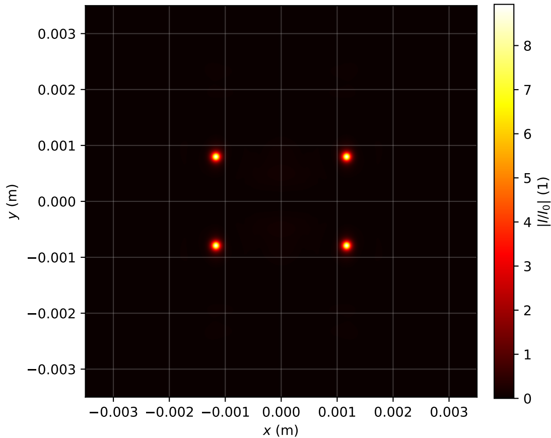
Intensity profile I(x, y, z = 2.946)/I_0 , P_{in}=7.0P_{cr} , artificial time
